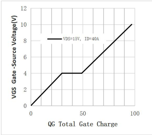
Fig.1 Gate-Charge Characteristics
