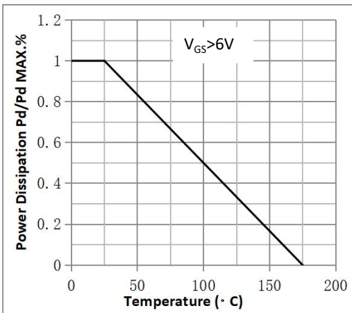
Fig.3 Power Dissipation
