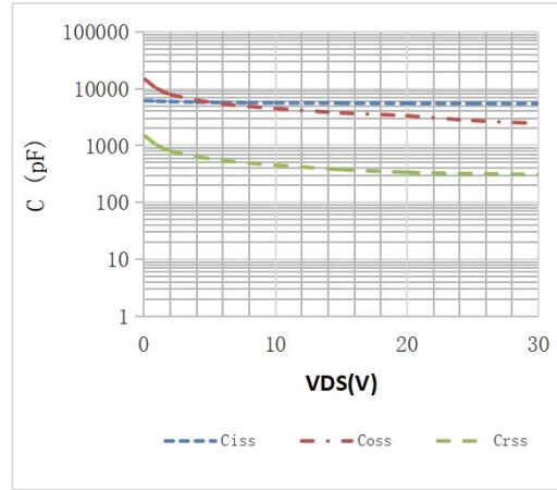
Fig.2 Capacitance Characteristics
